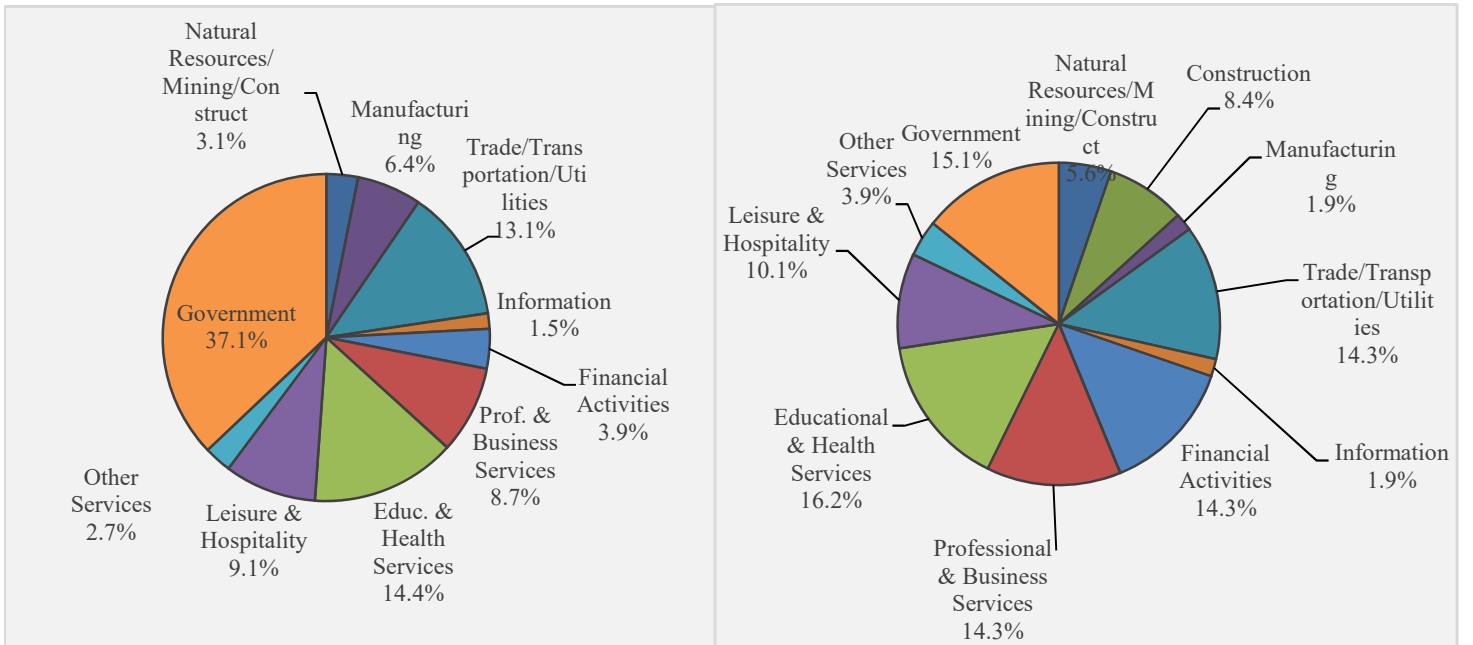
12-month Employment Change by Industry in the Champaign-Urbana Area (May - 2021)
